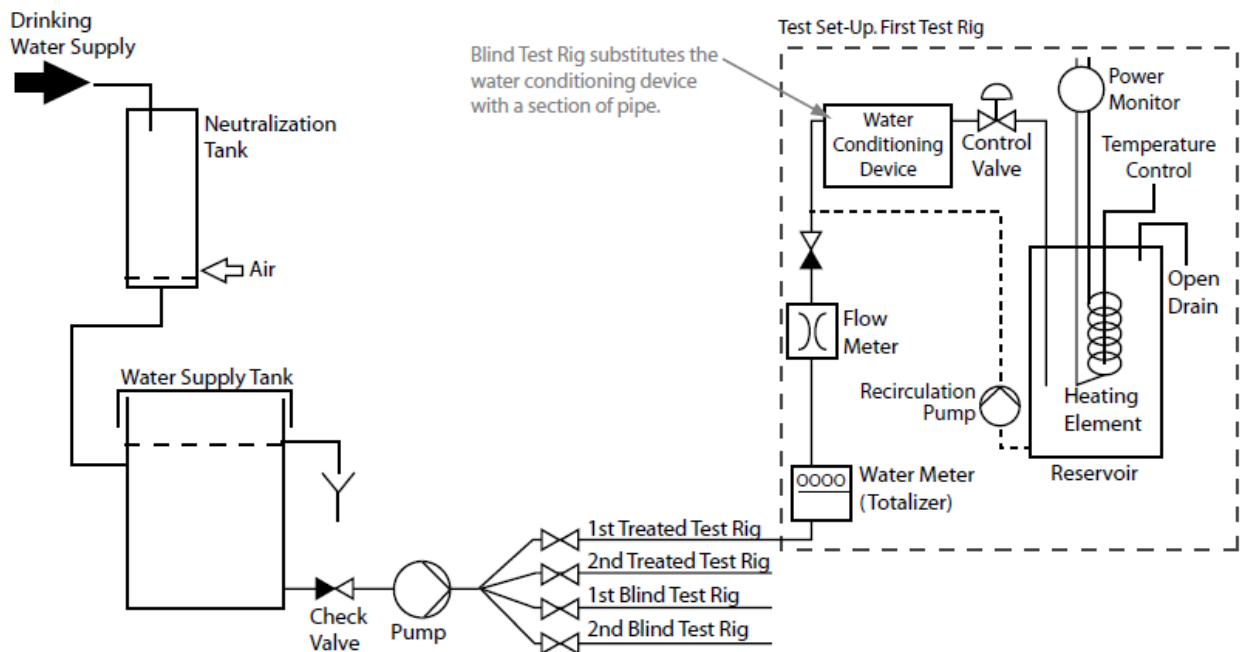
FIGURE 14: DVGW-W512 SCHEMATIC
